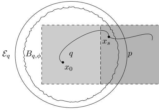
Fig. 3. Example trajectory for an interconnected system with a two-dimensional state space. The trajectory starts from x_0 , but the sampling delay \phi causes the input v to remain fixed to q even though the trajectory has entered the quantization region p . The update to v = p occurs at x_s instead of at the boundary between p and q . The sets \mathcal{E}_q and B_{q,\phi} over which the Lyapunov function V_q is valid are shown.
